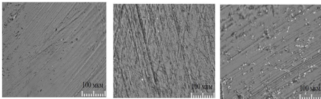
Fig. 4. General view of friction surfaces for pure PA-6 (a), PA-6 with 0.01 wt.% C60 fullerenes (b) and for PA-6 with 10 wt.% carbon fibers (c), obtained by polymerization in situ, x400
