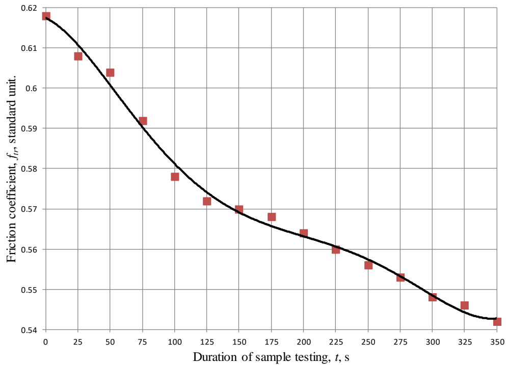
Fig. 2. Dynamics of changes in the coefficient of friction for samples of composite material: PA-6 filled with 10 wt.% carbon fibers, obtained by polymerization in situ
